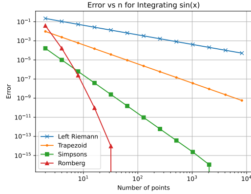
Figure 23: Example of Error for different methods for \sin x from a = 0, b = 1 . We see that asymptotically, Romberg performs much better compared with trapezoid and Riemann rule.
