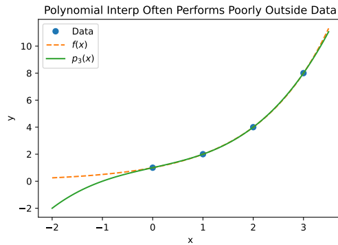
Figure 13: Data and interpolating polynomial from Example 18.3. Notice that the interpolating polynomial does not do well for extrapolating an exponential trend beyond its data.
