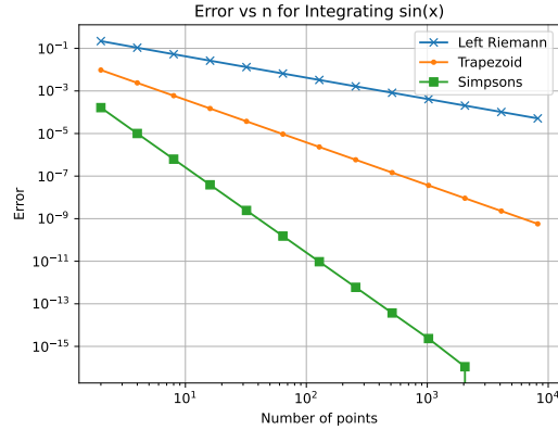
Figure 22: Example of Error for different methods for \sin x from a = 0, b = 1 . We see that asymptotically, Simpson performs much better compared with trapezoid and Riemann rule.
