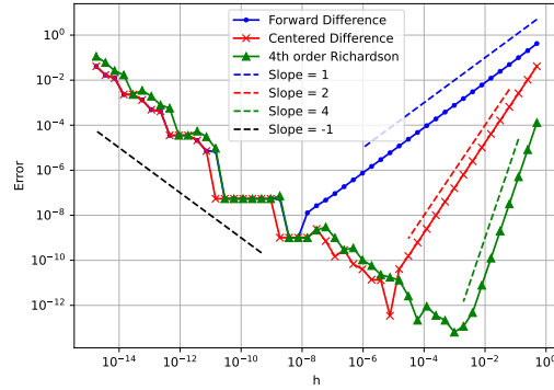
Figure 21: Relative error \frac{|f(x+h)-f(x)-f'(x)|}{|f'(x)|} vs h for f(x) = \sin(x) using forward difference, centered difference, and Richardson Extrapolation. Notice that the slope of each error curve is steeper the more accurate the formula.
