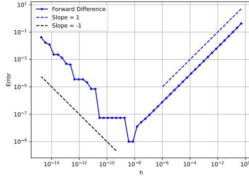
Figure 19: Relative error \frac{|f(x+h)-f(x)-f'(x)h|}{|f'(x)|} vs h for f(x) = \sin(x) . Notice that the error climbs after h \approx 10^{-8} due to floating point error.
