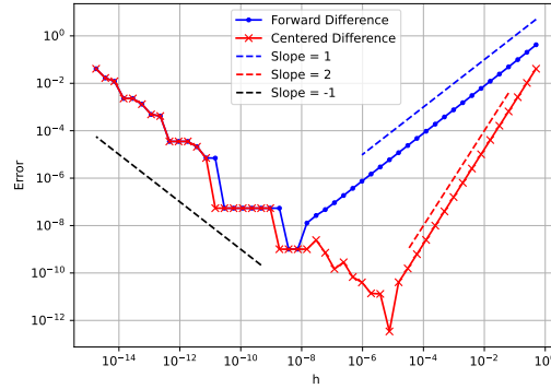
Figure 20: Relative error \frac{\left| \frac{f(x+h)-f(x)}{h} - f'(x) \right|}{|f'(x)|} vs h for f(x) = \sin(x) using forward and centered differences. Notice that the minimum error is smaller for centered differences but occurs for large h .
